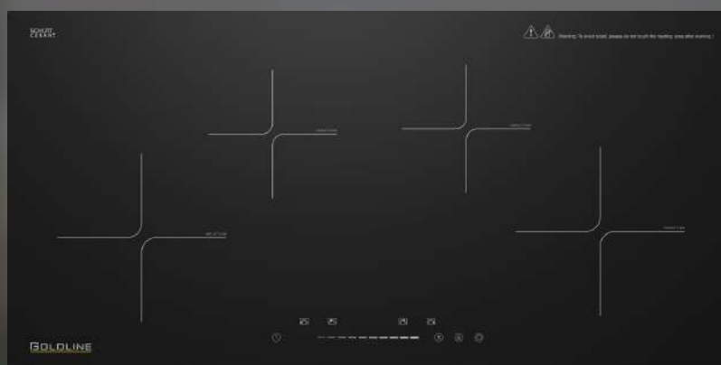
IH904CSAB Dimension: 900 x 520 MM (90CM) Cut-Out size: 880 x 430 MM Tray depth: 60 MM
